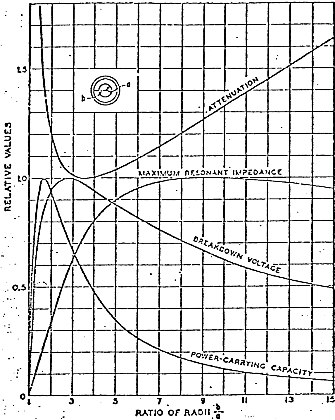
Various characteristics of a coaxial transmission line plotted as the ratio of radii of outer and inner conductors.
